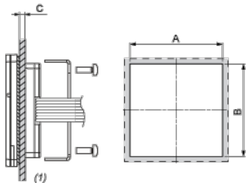
(1) Installation panel
